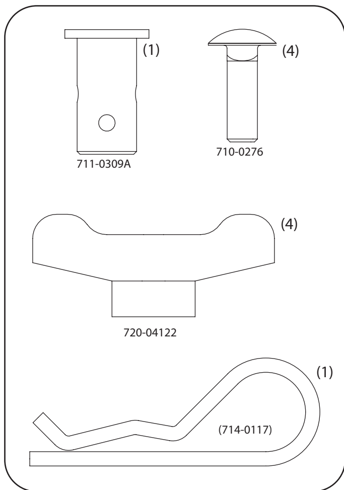
Hardware Pack 689-00328
